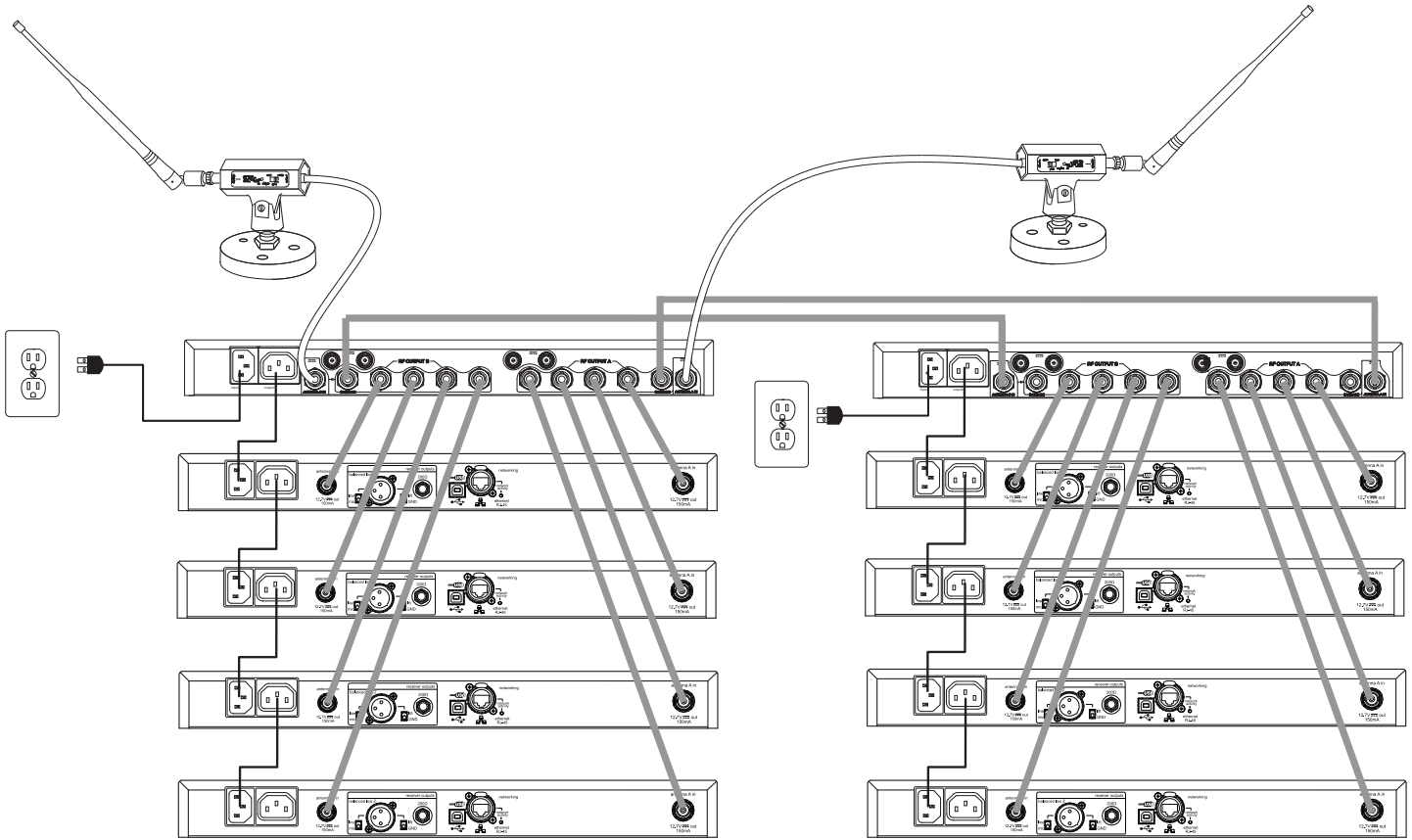
Multiple UA845UWB Setup
