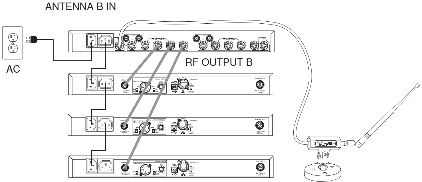
Single UA845UWB Setup
