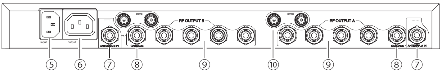
Rear Panel
